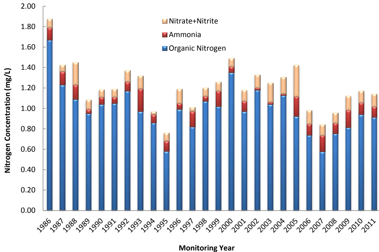
Figure 4.4 Average Nitrogen Concentrations Measured on the West Side of the Palmer Ranch from 1986 to 2011
