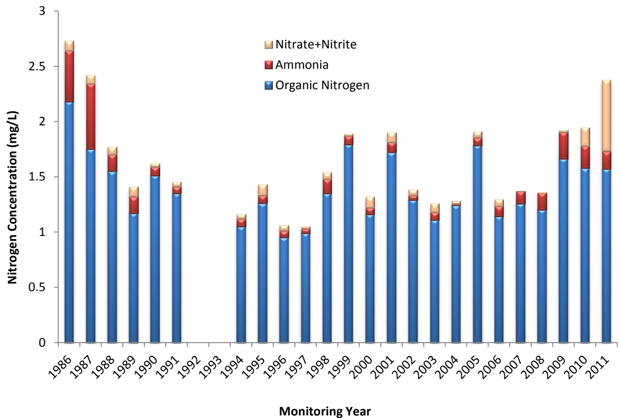
Figure 4.5 Average Nitrogen Concentrations Measured on the East Side of the Palmer Ranch from 1986 to 2011
