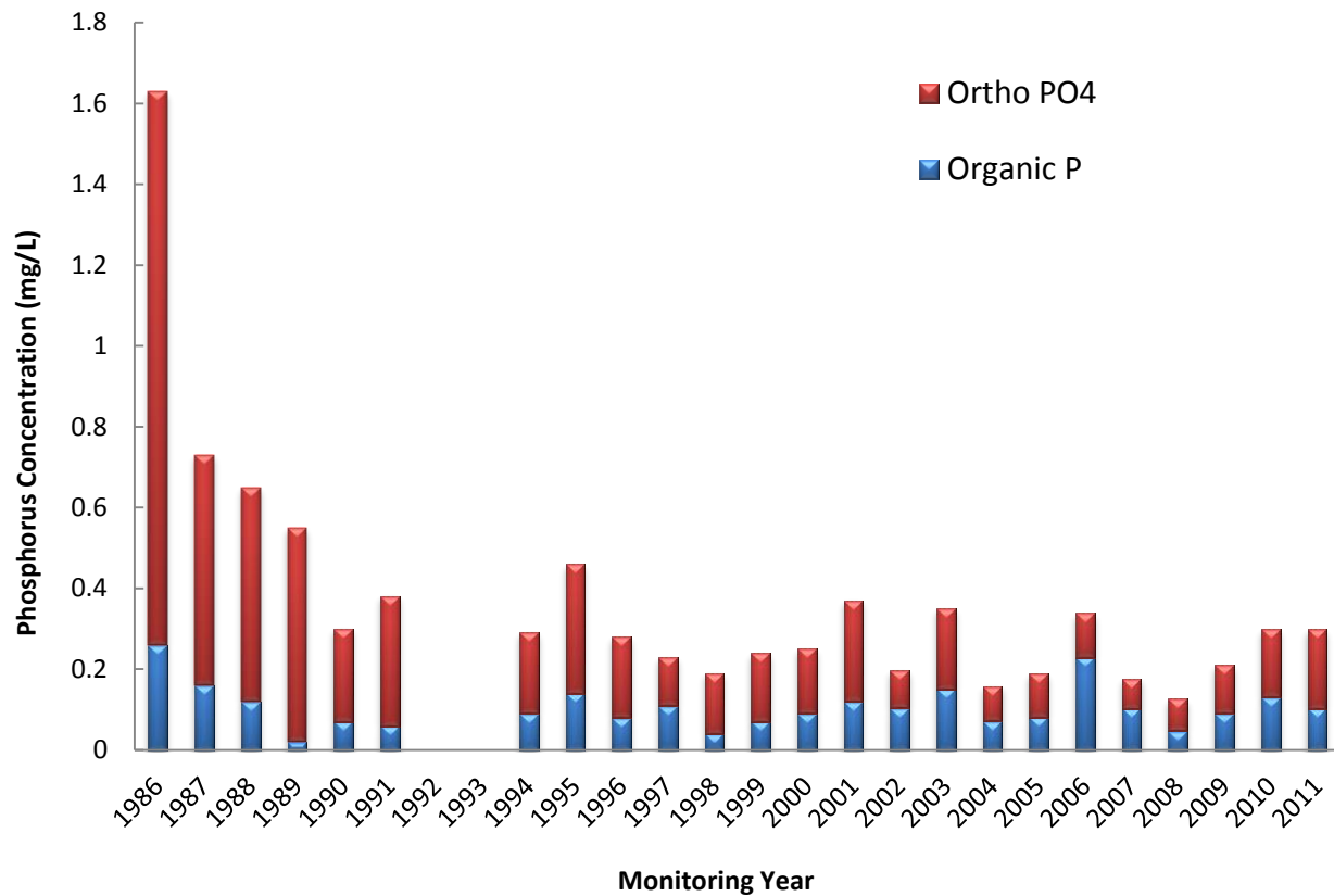
Figure 4.7 Average Phosphorus Concentrations Measured on the East Side of the Palmer Ranch from 1986 to 2011
