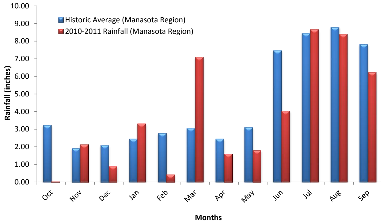
Figure 4.1 Historic Rainfall for the Period of Record and Average Rainfall for the Manasota Region for the Period October 2010 through September 2011
