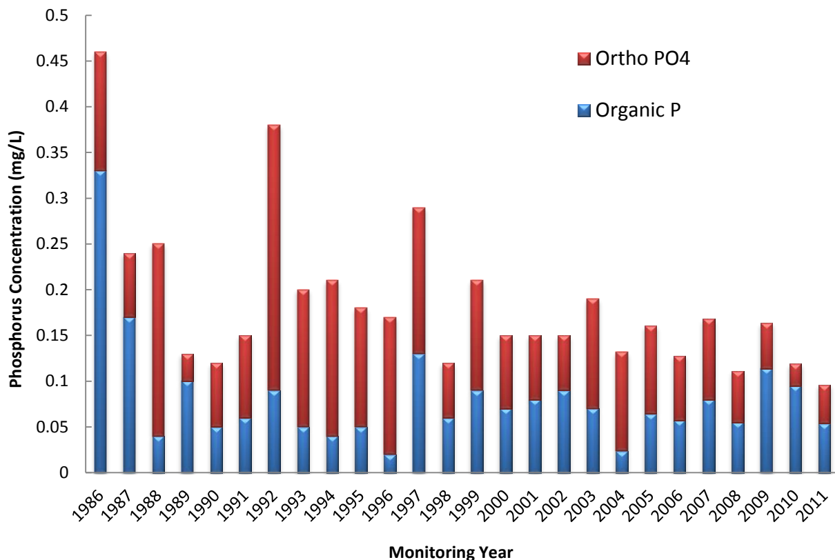
Figure 4.6 Average Phosphorus Concentrations Measured on the West Side of the Palmer Ranch from 1986 to 2011
