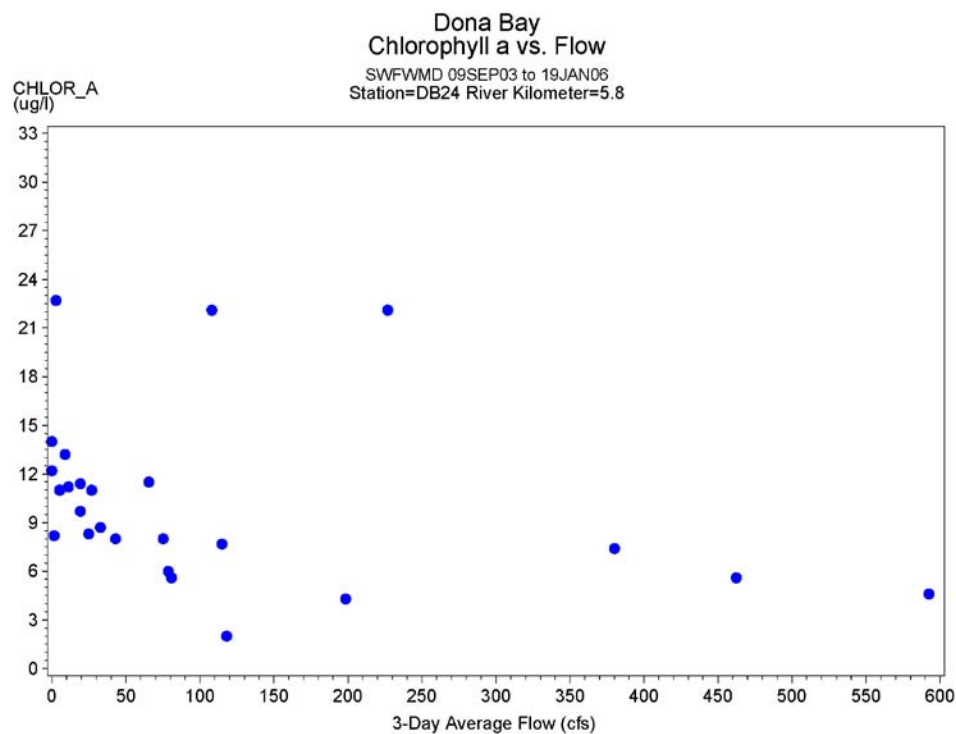
Figure 4-29. Dona Bay/Shakett Creek chlorophyll a versus flow, Station DB24, river km 5.8.
