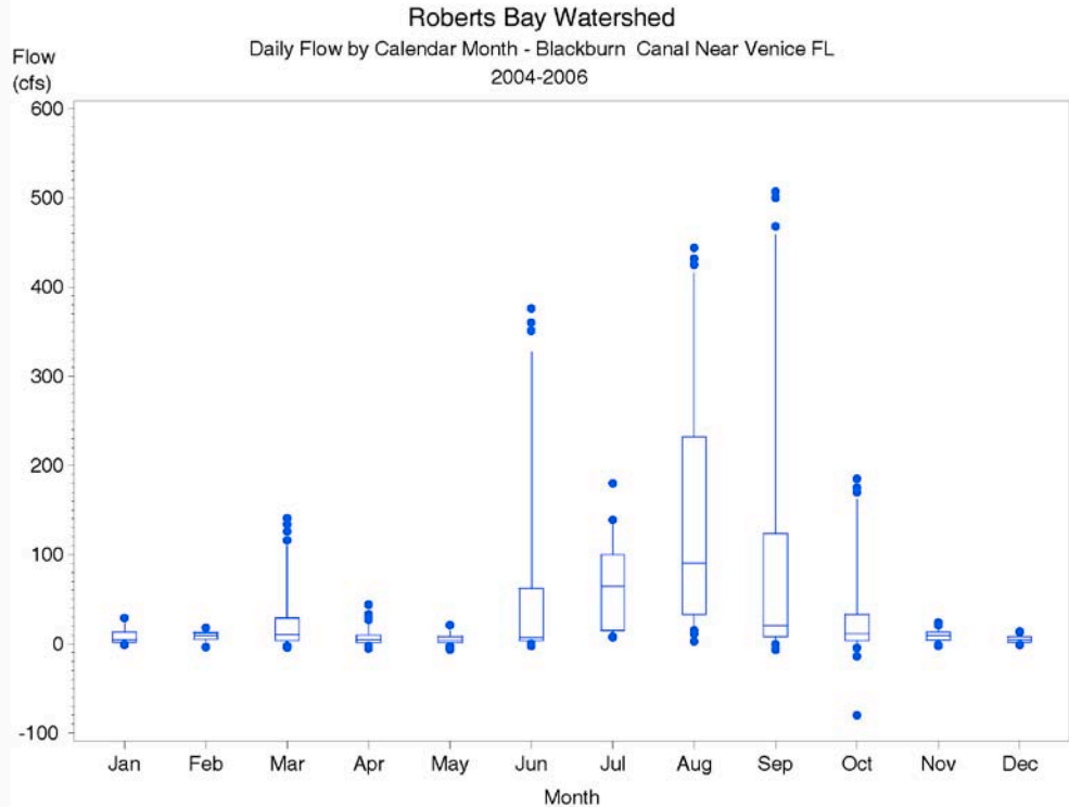
Figure 2-19. Box and whisker of measured daily flows (cfs) by calendar month at the Blackburn Canal near Venice gauge (USGS 02299692) for the period 2004 to 2006.
