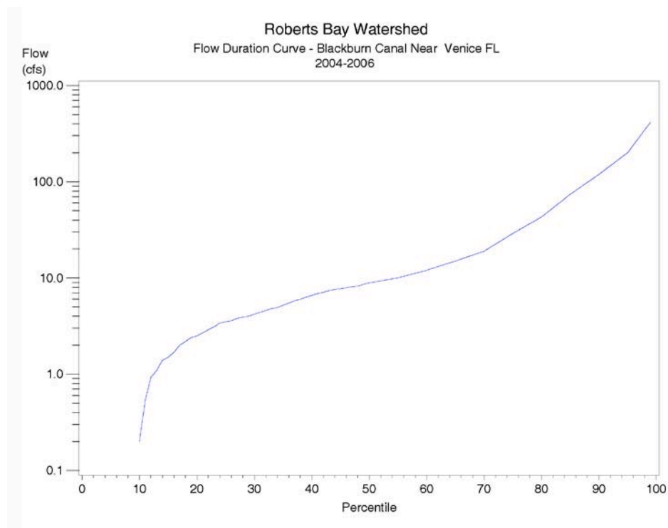
Figure 2-20. Flow duration curve of measured daily flows (cfs) at the Blackburn Canal near Venice gauge (USGS 02299692) for the period 2004 to 2006.
