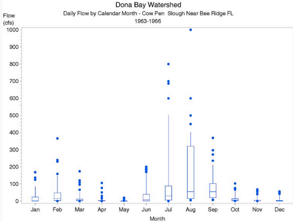
Figure 2-13. Box and whisker of measured daily flows (cfs) by calendar month at the Cow Pen Slough near Bee Ridge gauge (USGS 02299700) for the period from 1963 to 1966.
