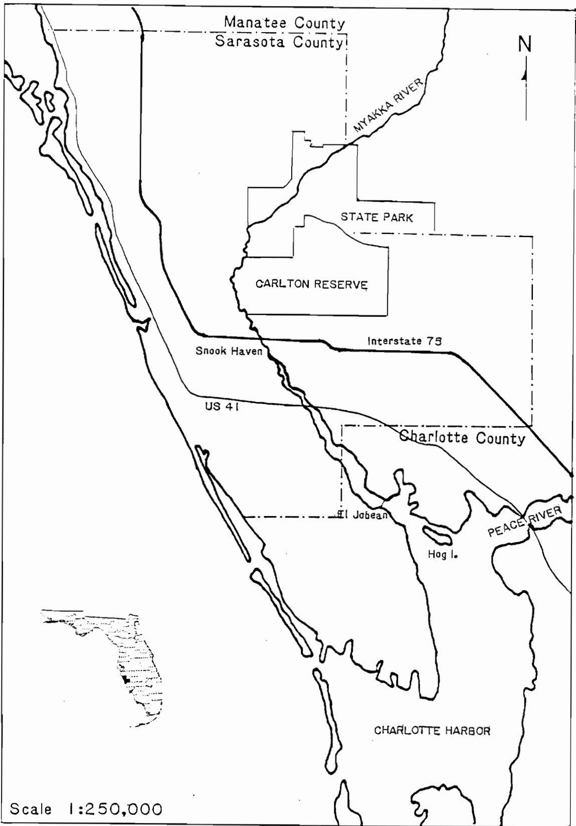
Figure 1. Location of the tidal Myakka River. The study area falls between Interstate 75 and the Sarasota-Charlotte County line.
