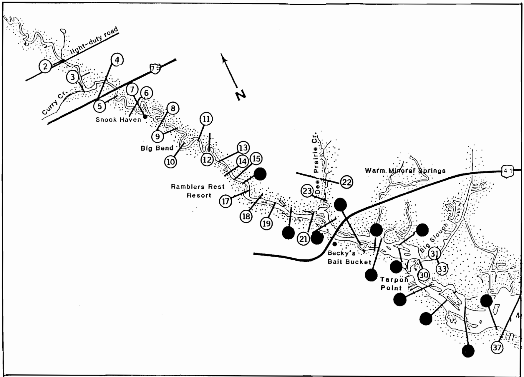
Figure 12. Distribution of widgeon grass in the tidal Myakka River, October 1987 to August 1988. Data from both banks were combined.
