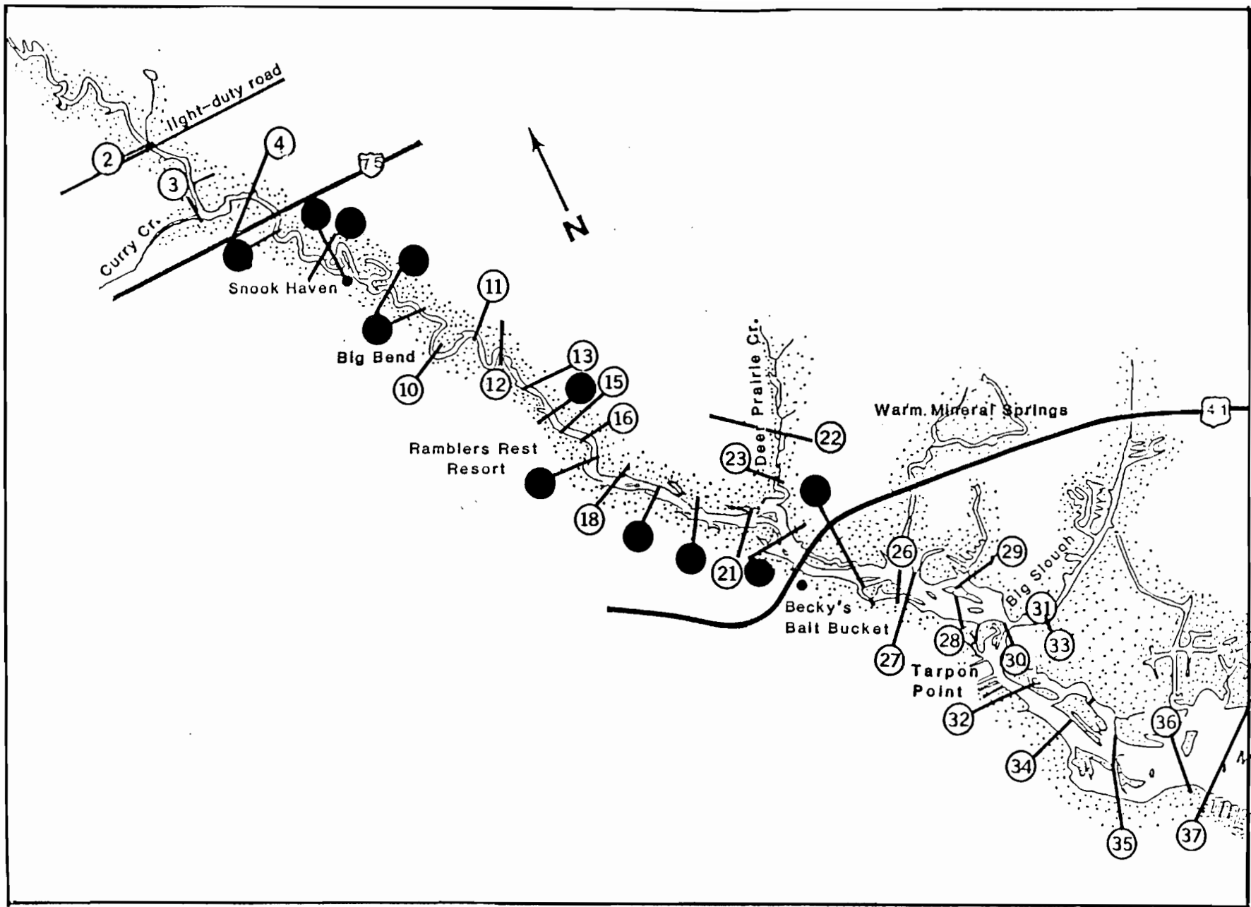
Figure 14. Distribution of dwarf arrowhead in the tidal Myakka River, October 1987 to August 1988. Data from both banks were combined.
